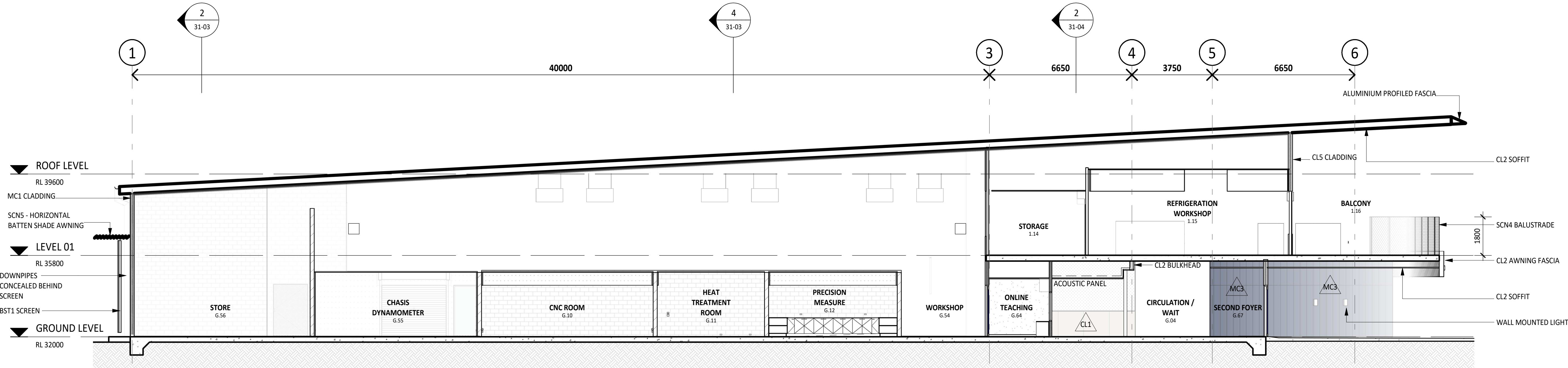
1 BUILDING SECTION - 6 21-01 1 : 100
