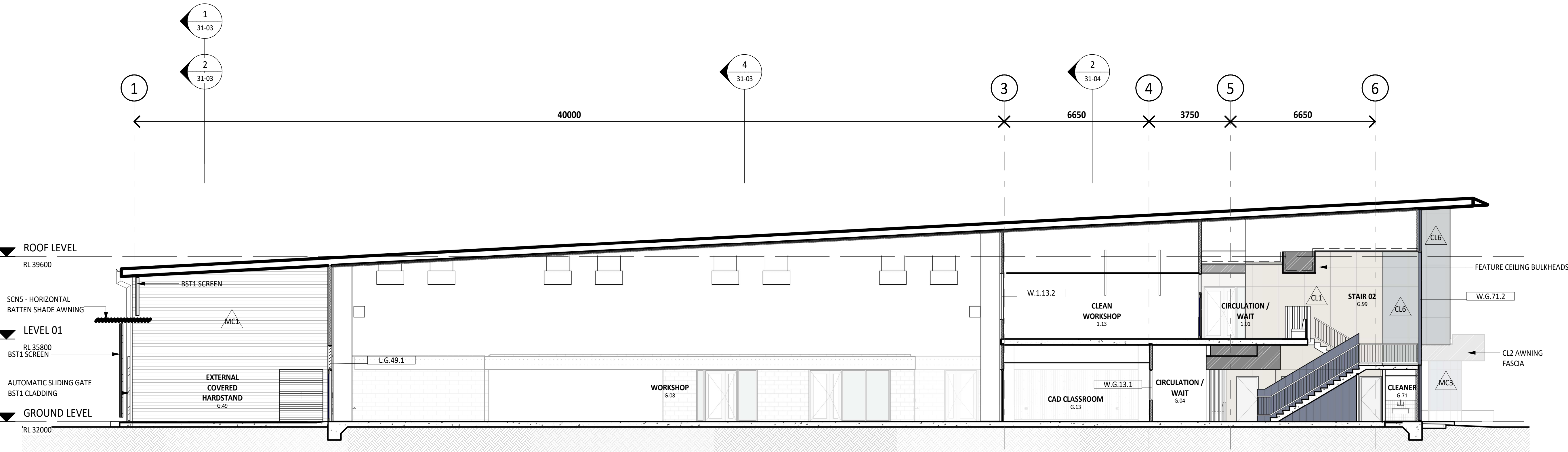
2 BUILDING SECTION - 7 21-02 1 : 100
